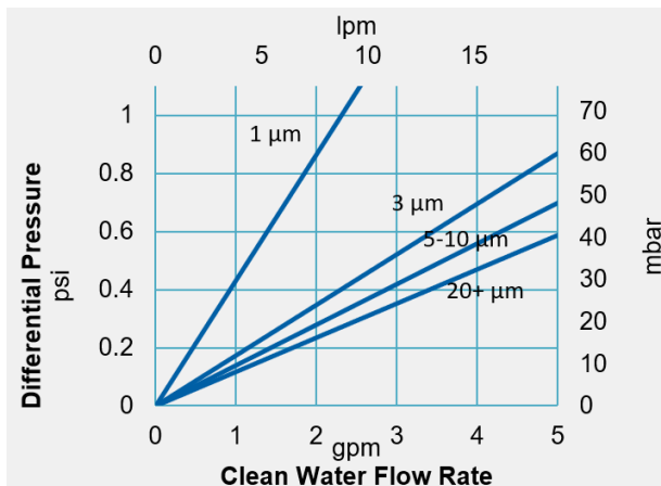
Graph 1: Purtrex PX clean water flow rate based on a 10 in length filter
